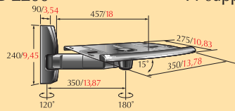
TVB 2200 TV support
