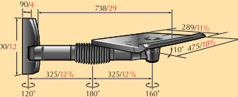
EFW 2350 TV support
