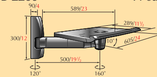
TVB 2260 TV support
