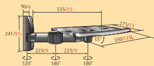
TVB 2225 TV support
