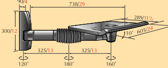
TVB 2360 TV support
