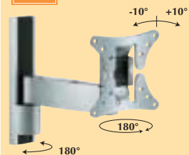
EFW 1020 LCD wall support
