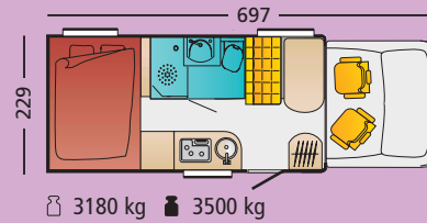
Delfin Performance t 700
