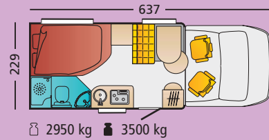
Delfin Performance t 625
