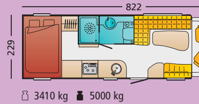
Delfin Performance t 821
