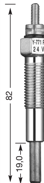
Y-771 R M 10 x 1.25 12 Hex 24 V
