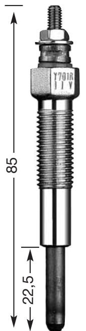
Y-701 R M 10 x 1.25 12 Hex 11 V
