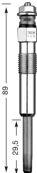
Y-503 R M 10 x 1.0 10 Hex 11 V DP 10
