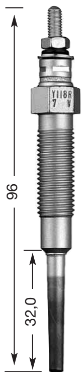
Y-118 R M 10 x 1.25 12 Hex 7 V
