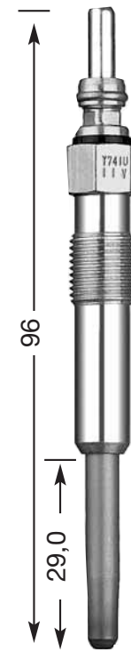
Y-741 U M 10 x 1.0 10 Hex 11 V DP 20
