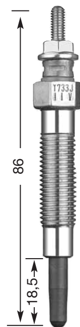
Y-733 J M 10 x 1.25 12 Hex 11 V DP 13
