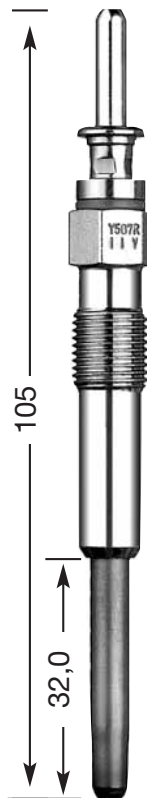
Y-507 R M 10 x 1.0 10 Hex 11 V DP 32
