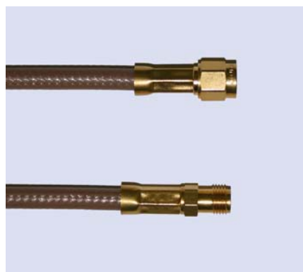
Kabel / Cable Anschluß Connector RG142B/U SMA-Stecker/SMA-Kuppler SMA male/SMA female
