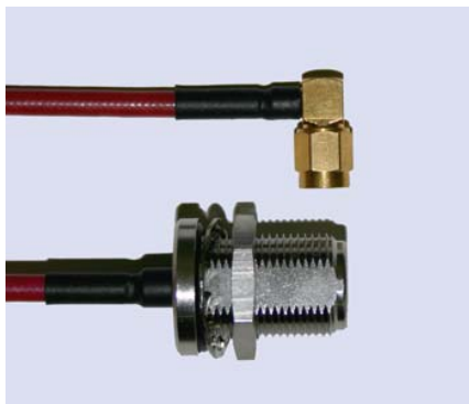
Kabel / Cable Anschluß Connector Succoform 141 FEP SMA-Winkelstecker/ N-Einbaukuppler SMA angle male/ N bulkhead female
