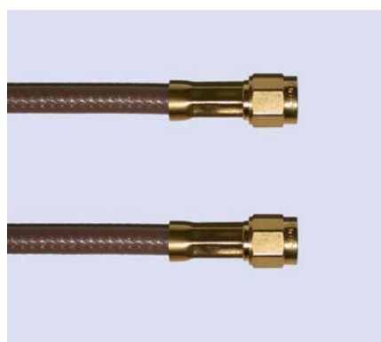
Kabel / Cable Anschluß Connector RG142B/U SMA-Stecker/SMA-Stecker SMA male/SMA male
