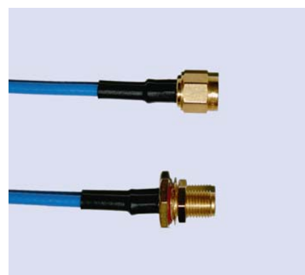
Kabel / Cable Anschluß Connector Multiflex 86 SMA-Stecker/SMA-Einbaukuppel SMA male/SMA bulkhead female
