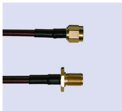
Kabel / Cable Anschluß Connector Succoform 86 FEP/PE SMA-Stecker/SMA-Einbaukuppler SMA male/SMA bulkhead female
