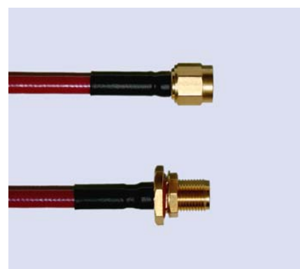
Kabel / Cable Anschluß Connector Succoform 141 FEP SMA-Stecker/SMA-Kuppler SMA male/SMA female
