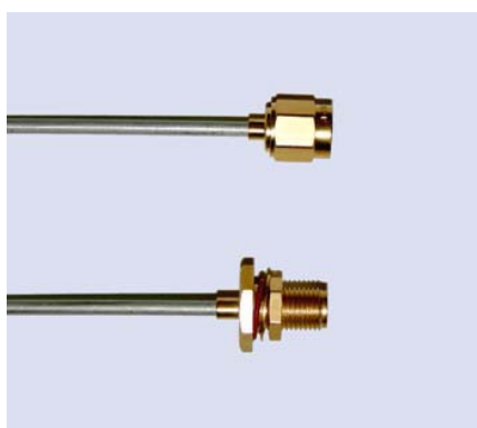
Kabel / Cable Anschluß Connector Semi Rigid UT 85 TP SMA-Stecker/SMA-Einbaukuppler SMA male/SMA female
