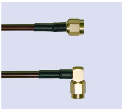
Kabel / Cable Anschluß Connector Succoform 86 FEP/PE SMA-Stecker/SMA-Winkelstecker SMA male/SMA angle male
