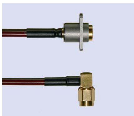
Kabel / Cable Anschluß Connector Succoform 86 FEP/PE BMA-Einbaukuppler/ SMA-Winkelstecker BMA bulkhead female/SMA angle male
