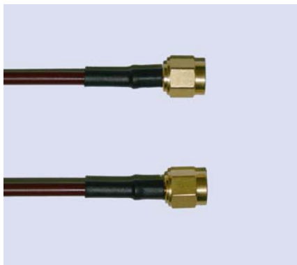
Kabel / Cable Anschluß Connector Succoform 86 FEP/PE SMA-Stecker/SMA-Stecker SMA male/SMA male
