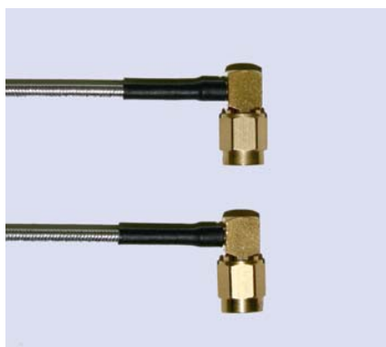
Kabel / Cable Anschluß Connector Succoform 141 SMA-Winkelstecker/SMA-Winkelstecker SMA angle male/SMA angle male
