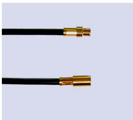
Kabel / Cable Anschluß Connector RG174A/U MCX-Stecker/MCX-Kuppler MCX male/MCX female
