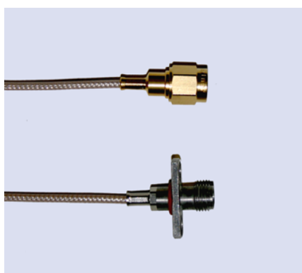
Kabel / Cable Anschluß Connector RG178 B/U SMA-Stecker/SMA-Einbaubuchse SMA male/SMA bulkhead female
