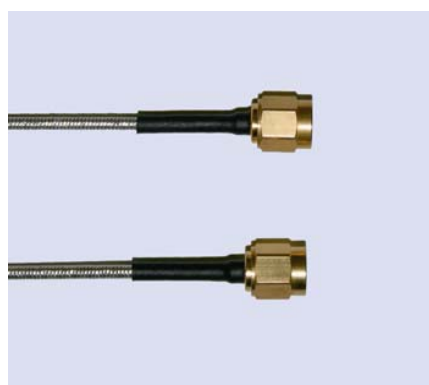
Kabel / Cable Anschluß Connector Succoform 86 SMA-Stecker/SMA-Stecker SMA male/SMA male
