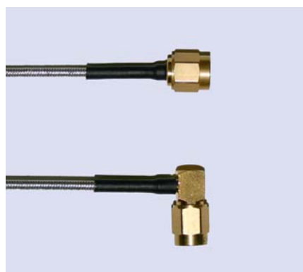
Kabel / Cable Anschluß Connector Succoform 141 SMA-Stecker/SMA-Winkelstecker SMA male/SMA angle male
