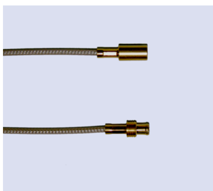
Kabel / Cable Anschluß Connector RG178 B/U MCX-Kuppler / MCX-Stecker MCX female/MCX male
