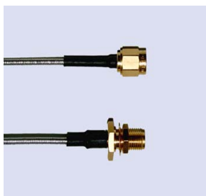
Kabel / Cable Anschluß Connector Succoform 86 SMA-Stecker/SMA-Einbaukuppler SMA male/SMA bulkhead female
