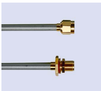
Kabel / Cable Anschluß Connector Semi Rigid UT 141 TP SMA-Stecker/SMA-Einbaukuppler SMA male/SMA female
