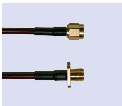
Kabel / Cable Anschluß Connector Succoform 86 FEP/PE SMA-Stecker/SMA-Kuppler m. Flansch SMA male/SMA bulkhead female
